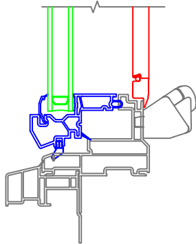
4-1/2 Banded Casing without J-Channel Standard Sill Nose
