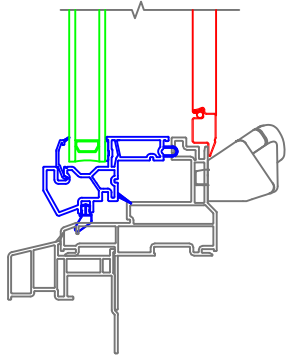
4-1/2 Banded Casing with J-Channel Standard Sill Nose
