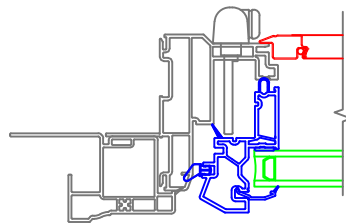
Brickmould Casing without J-Channel Standard Sill Nose
