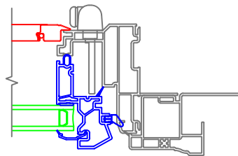
Brickmould Casing with J-Channel Historical Sill Nose
