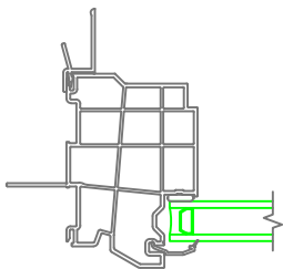
Without J-Channel
