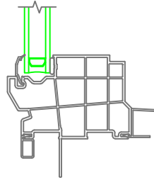
3/4" Drywall Return
