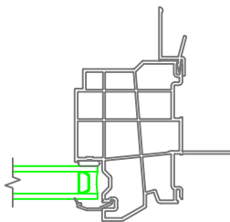
1/2"-5/8" Drywall Return
