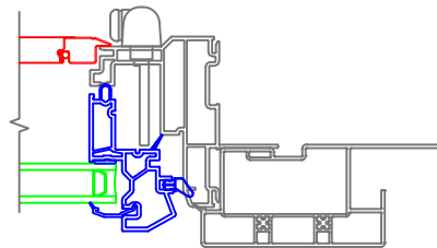
5/4 x 3-1/2 Flat Casing with J-Channel Historical Sill Nose
