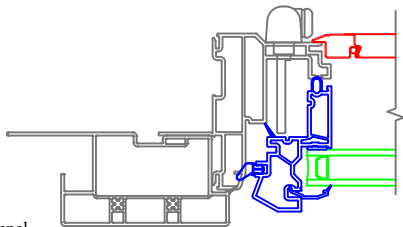
5/4 x 3-1/2 Flat Casing without J-Channel Standard Sill Nose
