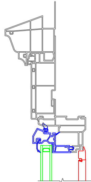
4-1/2 Banded Casing and Crown Crosshead Moulding
