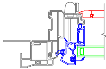
Brickmould Casing with J-Channel
