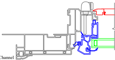
4-1/2 Banded Casing with J-Channel Standard Sill Nose
