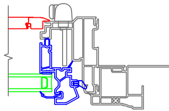
Brickmould Casing with J-Channel Historical Sill Nose
