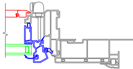
4-1/2 Banded Casing with J-Channel Historical Sill Nose
