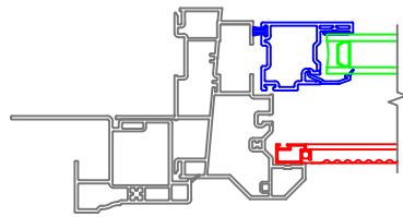
Brickmould Casing with J-Channel
