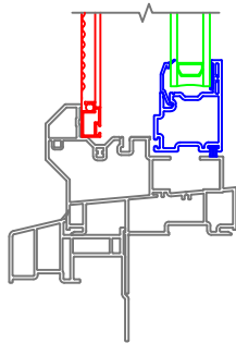
4-1/2 Banded Casing without J-Channel Standard Sill Nose
