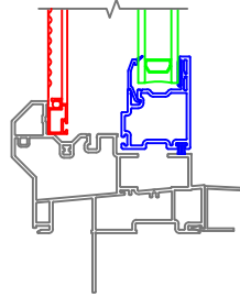
3/4" Drywall Return
