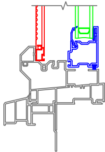
4-1/2 Banded Casing with J-Channel Standard Sill Nose
