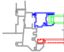
3/4" Drywall Return
