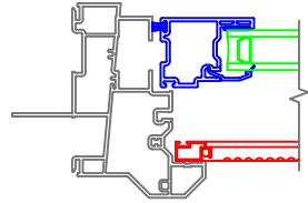
With J-Channel
