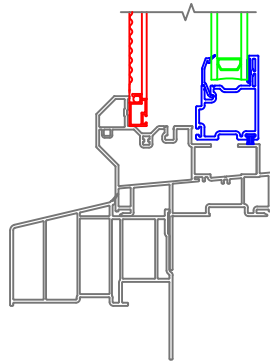
5/4 x 3-1/2 Flat Casing with J-Channel Historical Sill Nose
