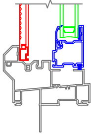
With J-Channel
