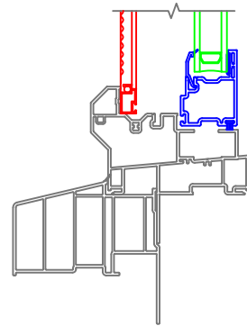
5/4 x 3-1/2 Flat Casing without J-Channel Historical Sill Nose
