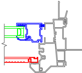
1/2"-5/8" Drywall Return
