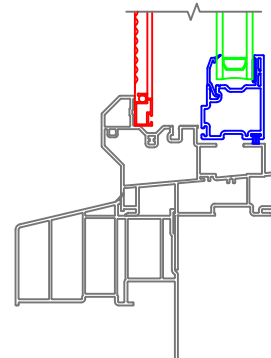
4-1/2 Banded Casing without J-Channel Historical Sill Nose
