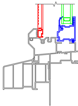
Brickmould Casing with J-Channel Historical Sill Nose
