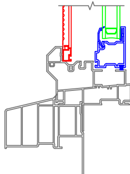
4-1/2 Banded Casing with J-Channel Historical Sill Nose
