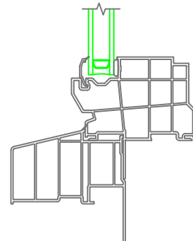
4-1/2 Banded Casing without J-Channel Historical Sill Nose
