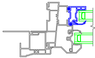
Brickmould Casing with J-Channel
