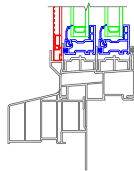
5/4 x 3-1/2 Flat Casing without J-Channel Standard Sill Nose
