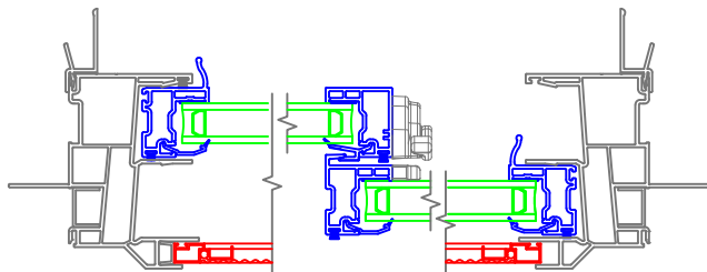
1/2"-5/8" Drywall Return
