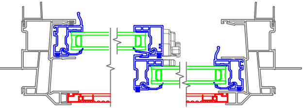
3/4" Drywall Return
