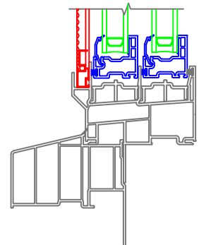
4-1/2 Banded Casing without J-Channel Historical Sill Nose
