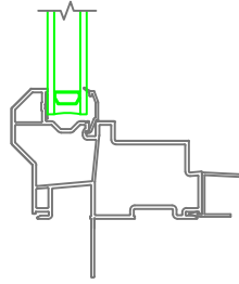
3/4" Drywall Return
