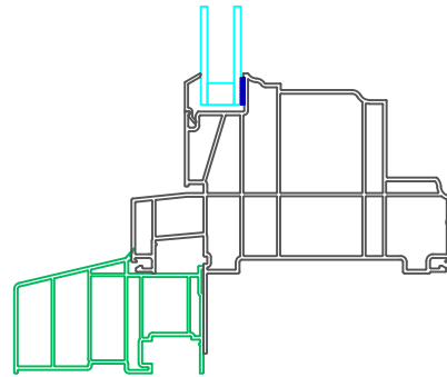
Brickmould Casing With Nailing Fin Removed Historical Sill Nose
