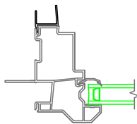
3/4" Drywall Return
