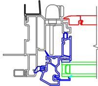
3/4" Drywall Return
