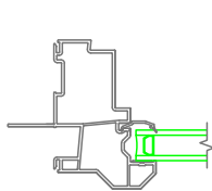
With J-Channel
