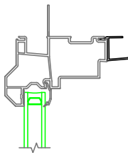
3/4" Drywall Return
